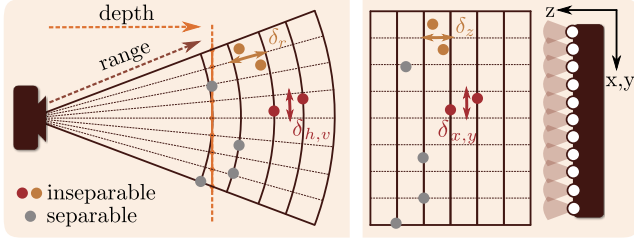
Fig. 3. Visualization of the effects caused by limited spatial resolution for multiple point targets. Optical sensors (left) divide spatial resolution into range resolution, \delta_r , and perspective pixel resolution, \delta_{h,v} . Contrary to that, near-field imaging radars (right) refer to range \delta_z and cross-range \delta_{x,y} resolution. We assume \delta_z \approx \delta_r and \delta_{x,y} \approx \delta_{h,v} for the sensor center, yet emphasize the conceptual difference between range and depth.
