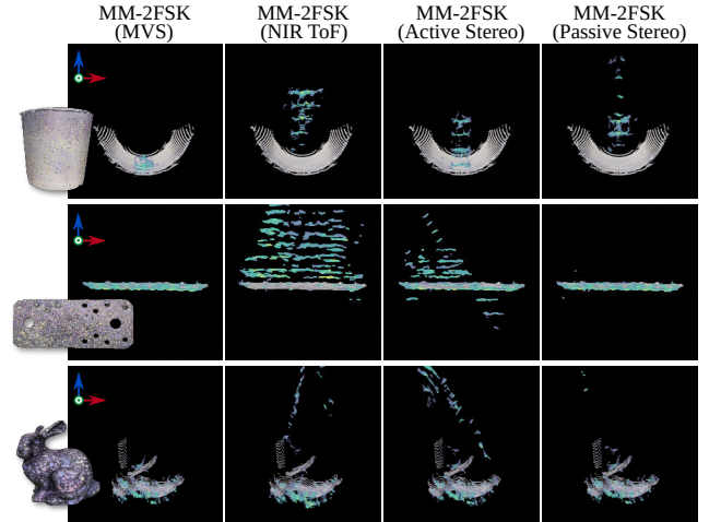
Fig. 8. Top-down views of the RF ToF reconstructions obtained with the MM-2FSK method, fused with the ground-truth MVS point cloud. Left to right: we vary the supporting sensor providing the depth prior. Top to bottom: we display the Flowerpot (Transparent) , V2 Metal Plate , and Bunny objects.
